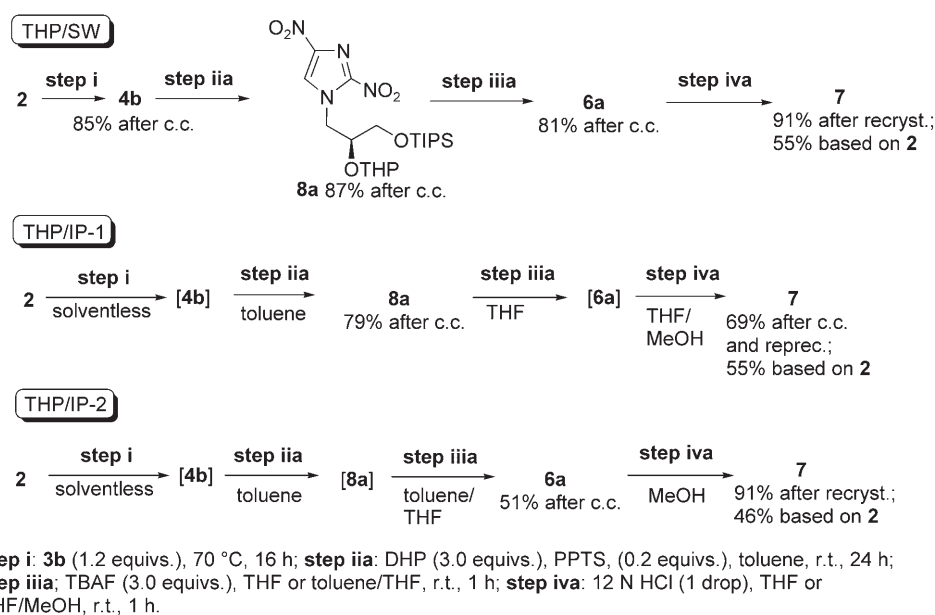
Scheme 2. THP route initiated by solventless reaction (for abbreviations, see Scheme 1).
