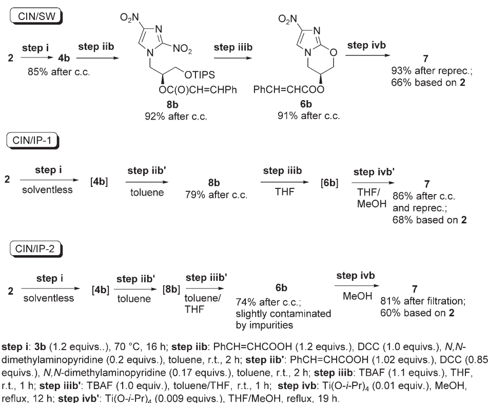
Scheme 3. Cinnamate route initiated by solventless reaction (for abbreviations, see Scheme 1).
