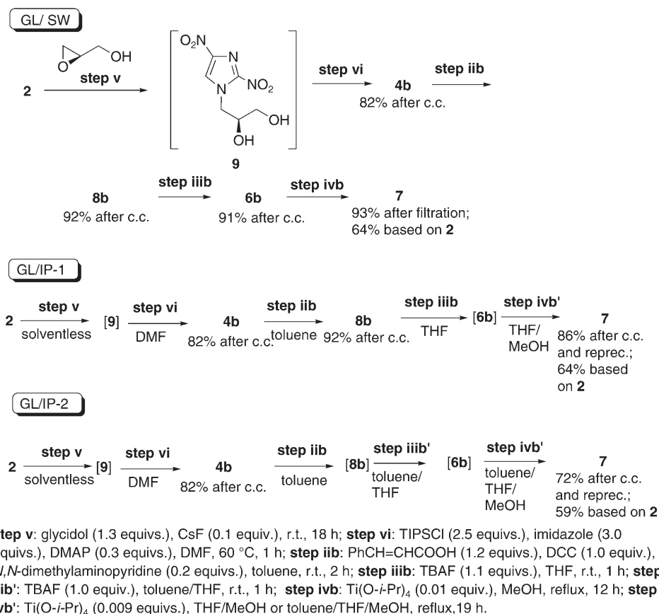
Scheme 4. Glycidol route initiated by solventless reaction (for abbreviations, see Scheme 1).
