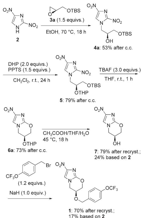
Scheme 1. PG process. DHP= dihydropyran; PPTS= pyridinium p -toluenesulfonate; TBAF= \text{Bu}_4\text{NF} ; r.t.= room temperature; c.c.= column chromatography; recryst.= recrystallization.
